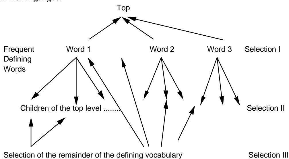
Figure 1: The selection of the first subset of the vocabulary
