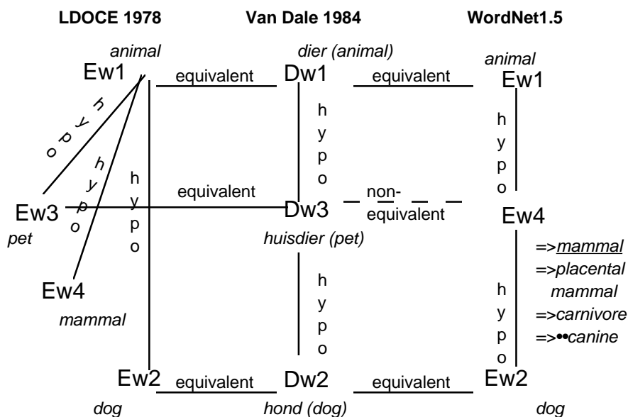
Figure 3: Variation in lexical configurations across wordnets
